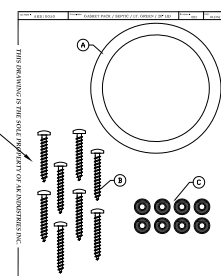
20" LID (LIDS WITH GASKETS INCLUDED WITH TANK)
