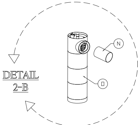
(OPTIONAL) OUTLET FILTER ASSEMBLY 2-B
