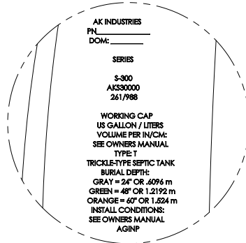
DETAIL 2-B
